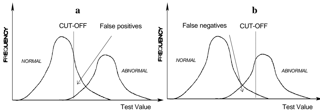
Figure 3: Effect of changing cut-off values on sensitivity and specificity
