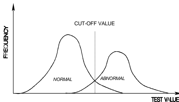
Figure 2: Distribution of test values for normal and abnormal populations
